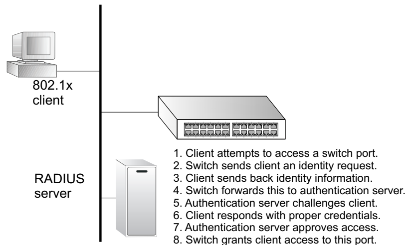
Figure 223: Configuring Port Authentication
