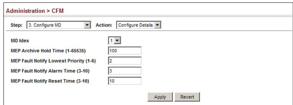
Figure 341: Configuring Detailed Settings for Maintenance Domains
