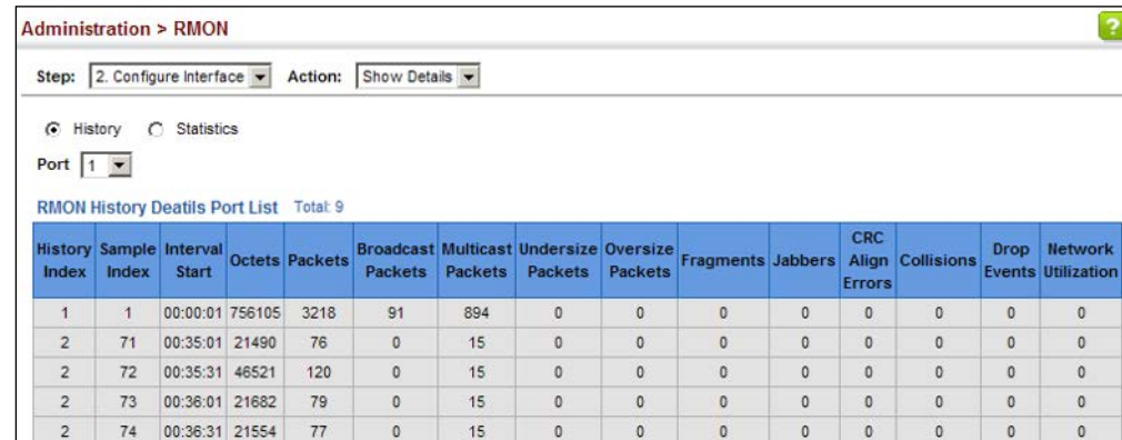
Figure 306: Showing Collected RMON History Samples
