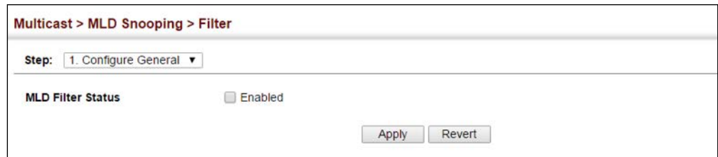
Figure 412: Enabling MLD Filtering and Throttling
