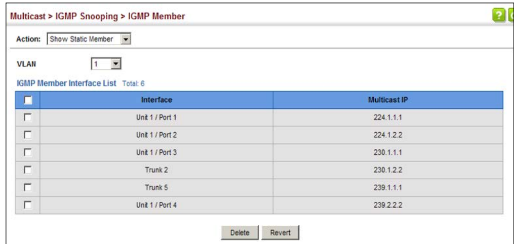
Figure 381: Showing Static Interfaces Assigned to a Multicast Service
