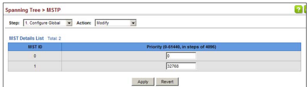
Figure 136: Modifying the Priority for an MST Instance
