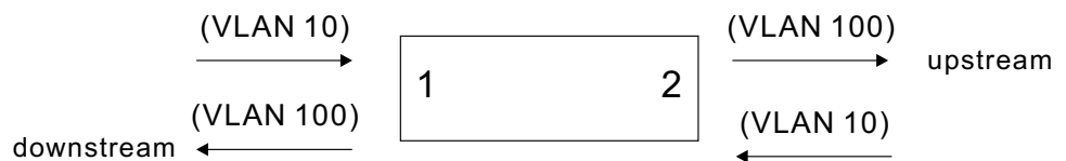
Figure 109: Configuring VLAN Translation
