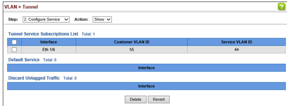
Figure 95: Showing CVLAN to SPVLAN Mapping Entries
