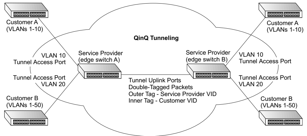
Figure 92: QinQ Operational Concept
