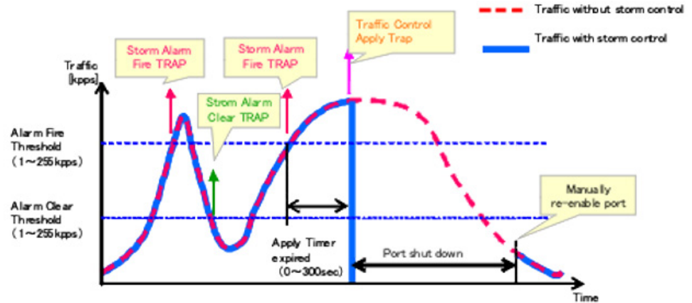
Figure 145: Storm Control by Shutting Down a Port
