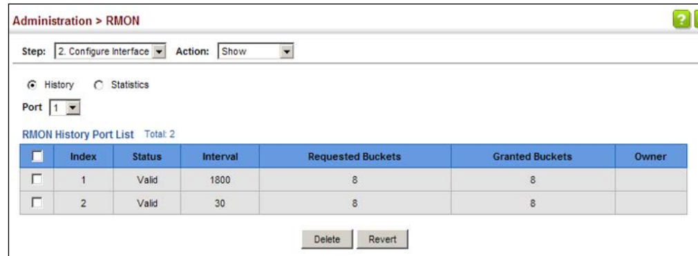
Figure 305: Showing Configured RMON History Samples
