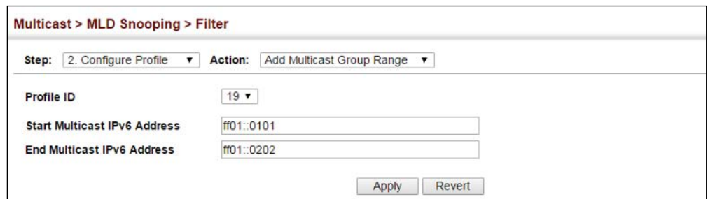
Figure 415: Adding Multicast Groups to an MLD Filtering Profile
