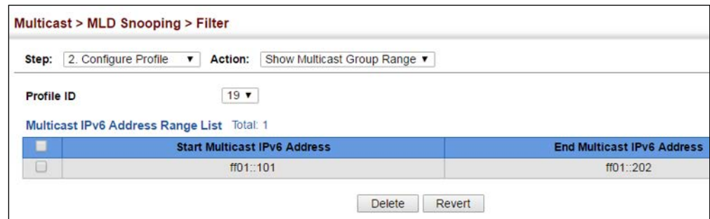
Figure 416: Showing the Groups Assigned to an MLD Filtering Profile
