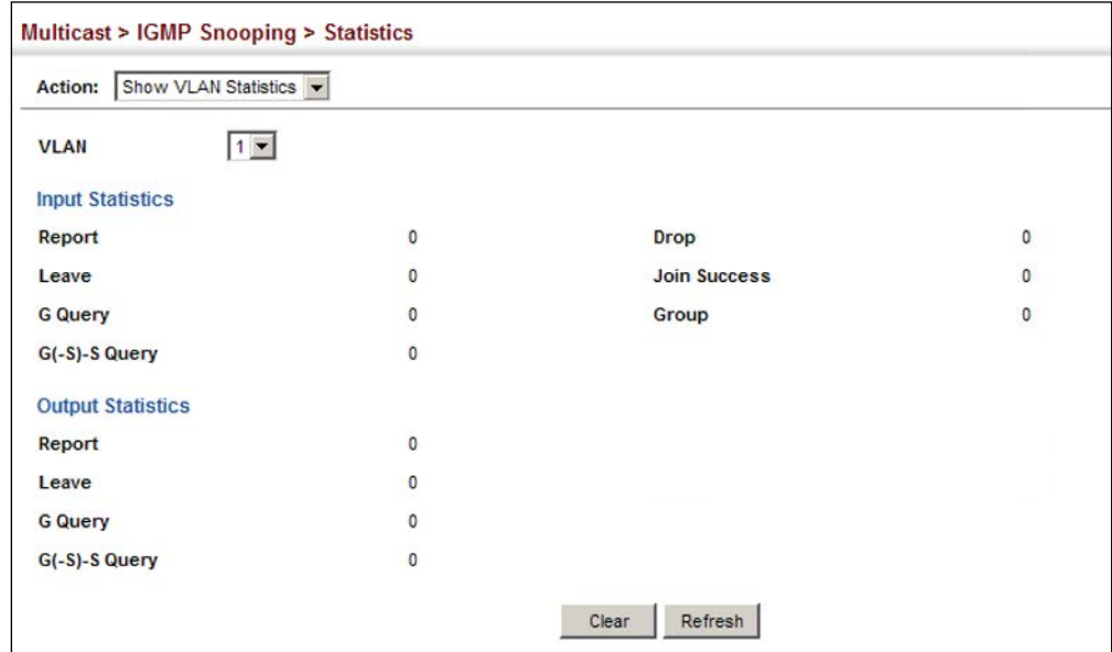
Figure 387: Displaying IGMP Snooping Statistics – VLAN
