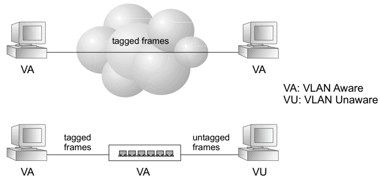
Figure 80: VLAN Compliant and VLAN Non-compliant Devices
