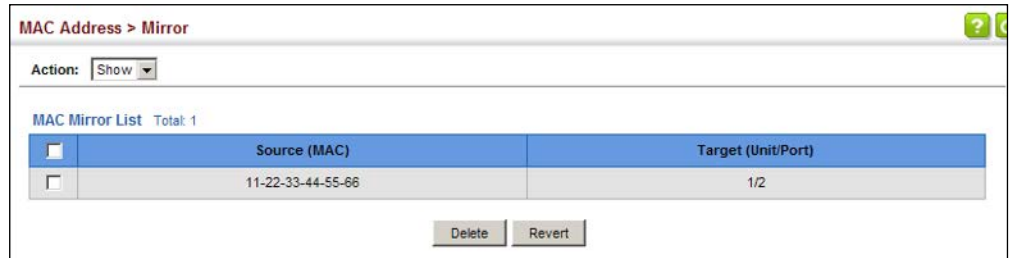
Figure 119: Showing the Source MAC Addresses to Mirror
