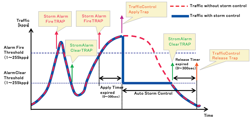
Figure 144: Storm Control by Limiting the Traffic Rate
