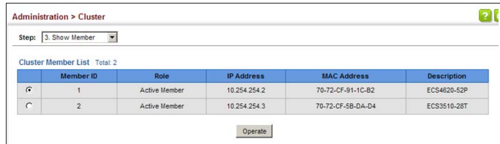
Figure 314: Managing a Cluster Member
