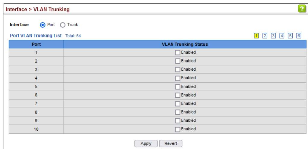
Figure 79: Configuring VLAN Trunking
