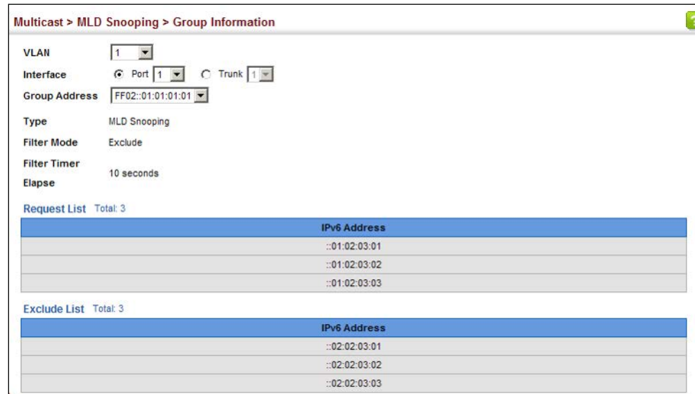
Figure 405: Showing IPv6 Multicast Services and Corresponding Sources
