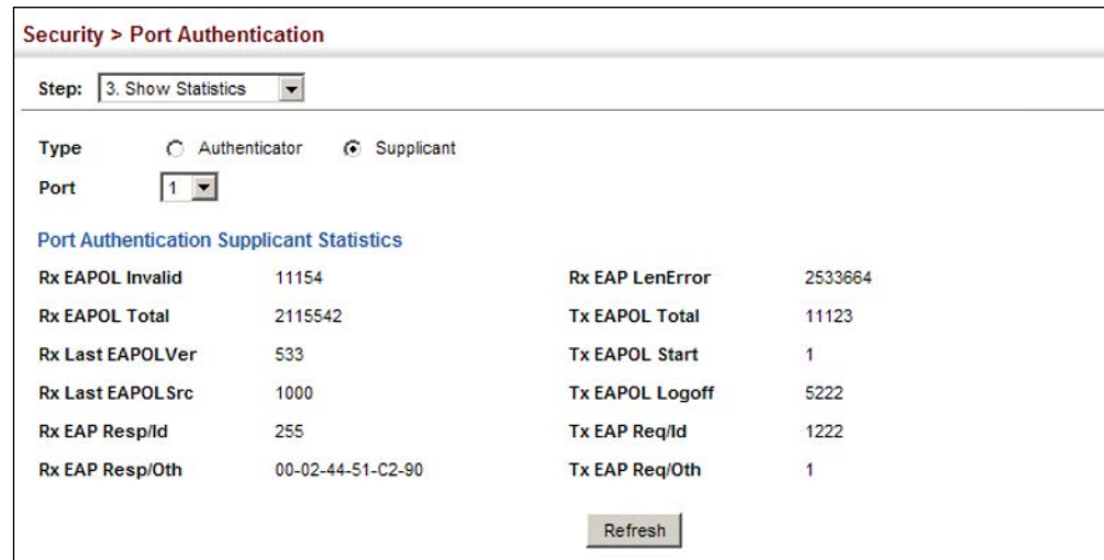
Figure 228: Showing Statistics for 802.1X Port Supplicant
