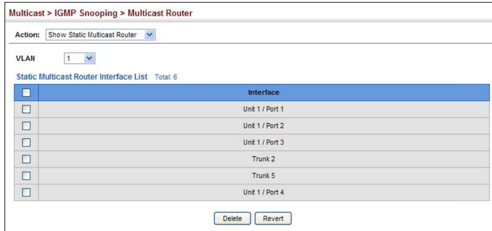
Figure 378: Showing Static Interfaces Attached a Multicast Router
