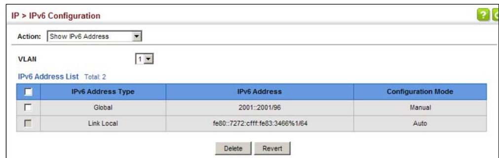
Figure 462: Showing Configured IPv6 Addresses
