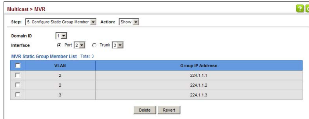
Figure 427: Showing the Static MVR Groups Assigned to a Port
