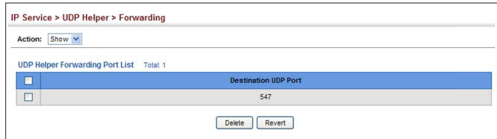
Figure 497: Showing the UDP Destination Ports
