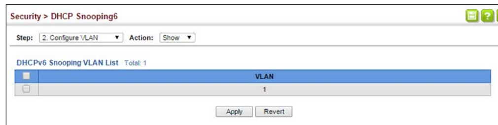
Figure 237: Showing VLANs Enabled for DHCPv6 Snooping
