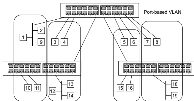
Figure 81: Using GVRP
