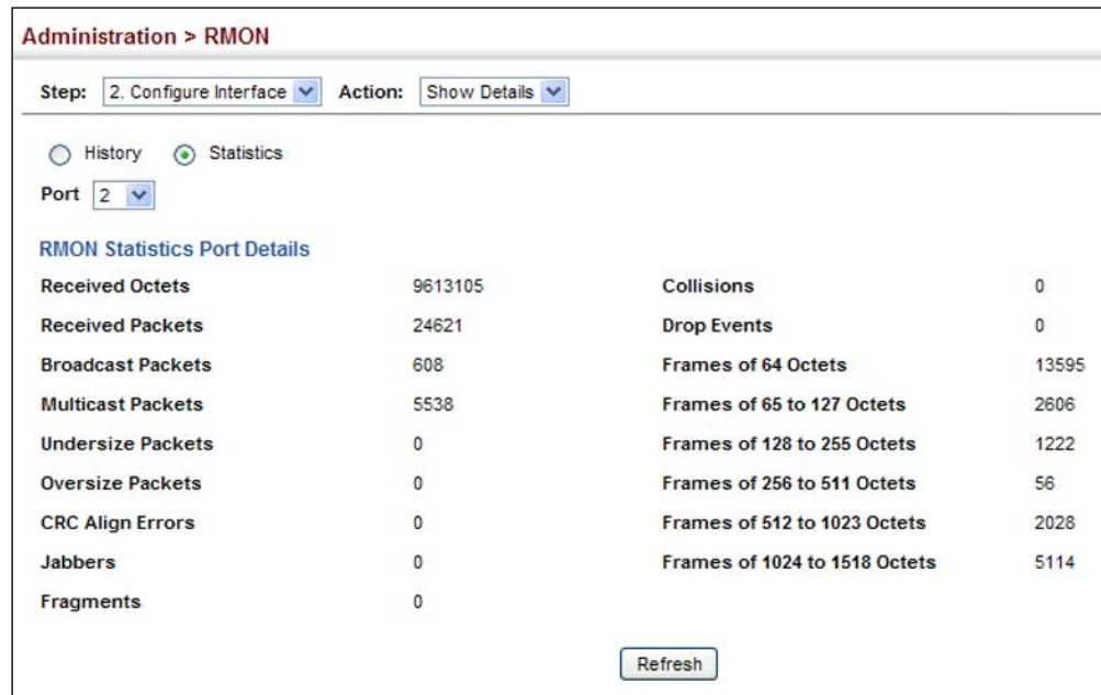
Figure 309: Showing Collected RMON Statistical Samples
