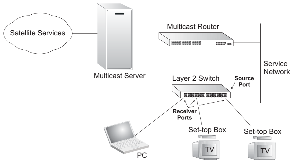
Figure 378: MVR Concept
