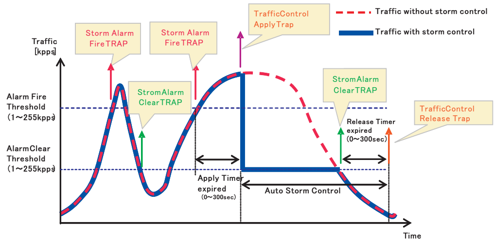
Figure 142: Storm Control by Limiting the Traffic Rate
