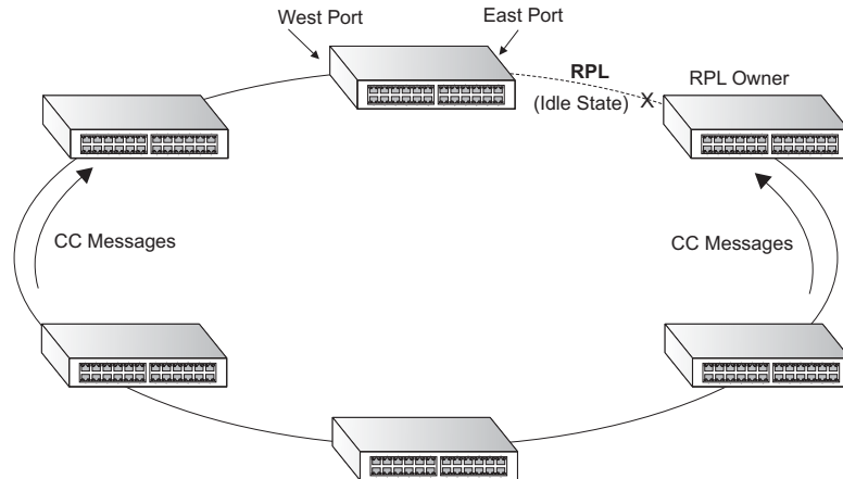
Figure 311: ERPS Ring Components
