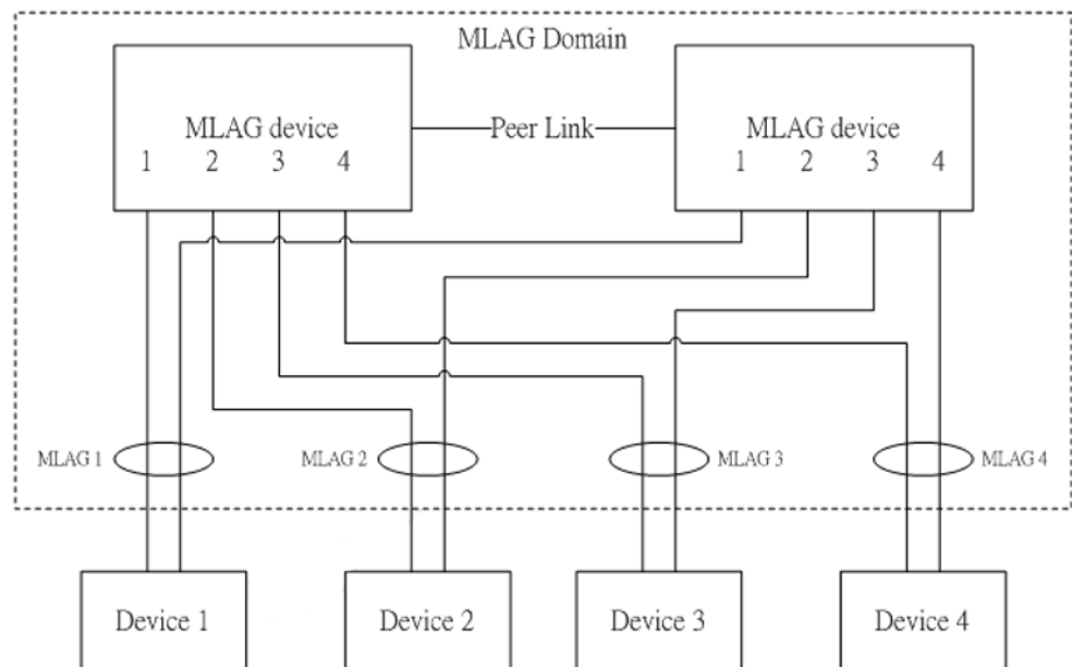
Figure 322: MLAG Domain Topology
