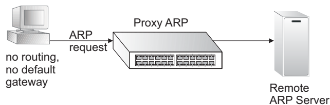
Figure 394: Proxy ARP
