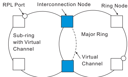
Figure 316: Sub-ring with Virtual Channel
