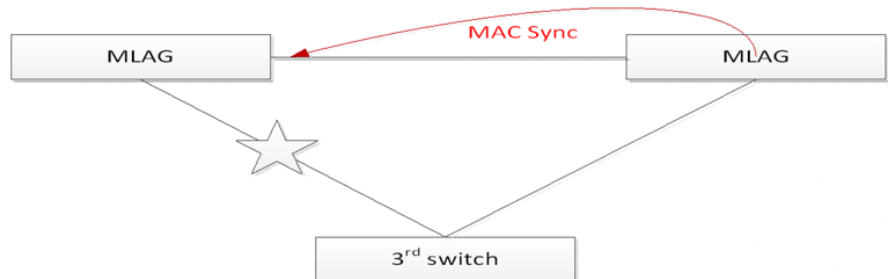
Figure 325: MLAG Peer Operation
