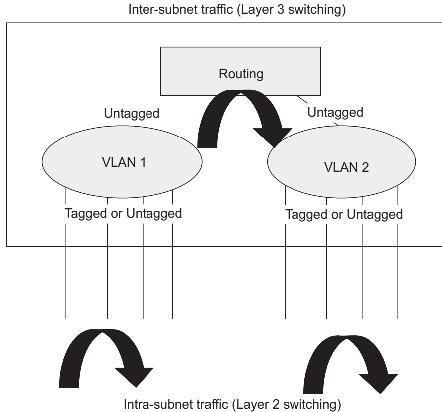
Figure 415: Virtual Interfaces and Layer 3 Routing
