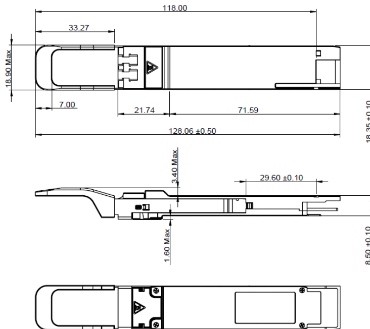
Figure 5. Mechanical Outline
